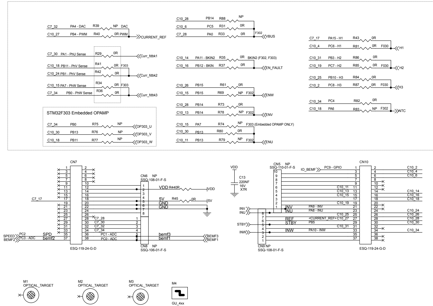
Figure 3. X-NUCLEO-IHM16M1 circuit schematic (3 of 5)
