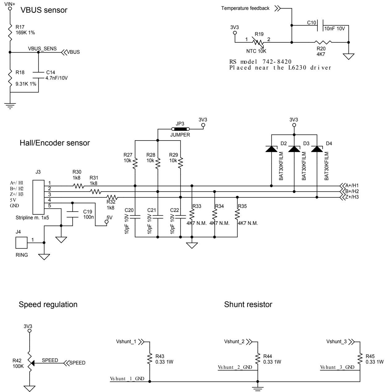
Figure 2. X-NUCLEO-IHM07M1 circuit schematic (2 of 4)
