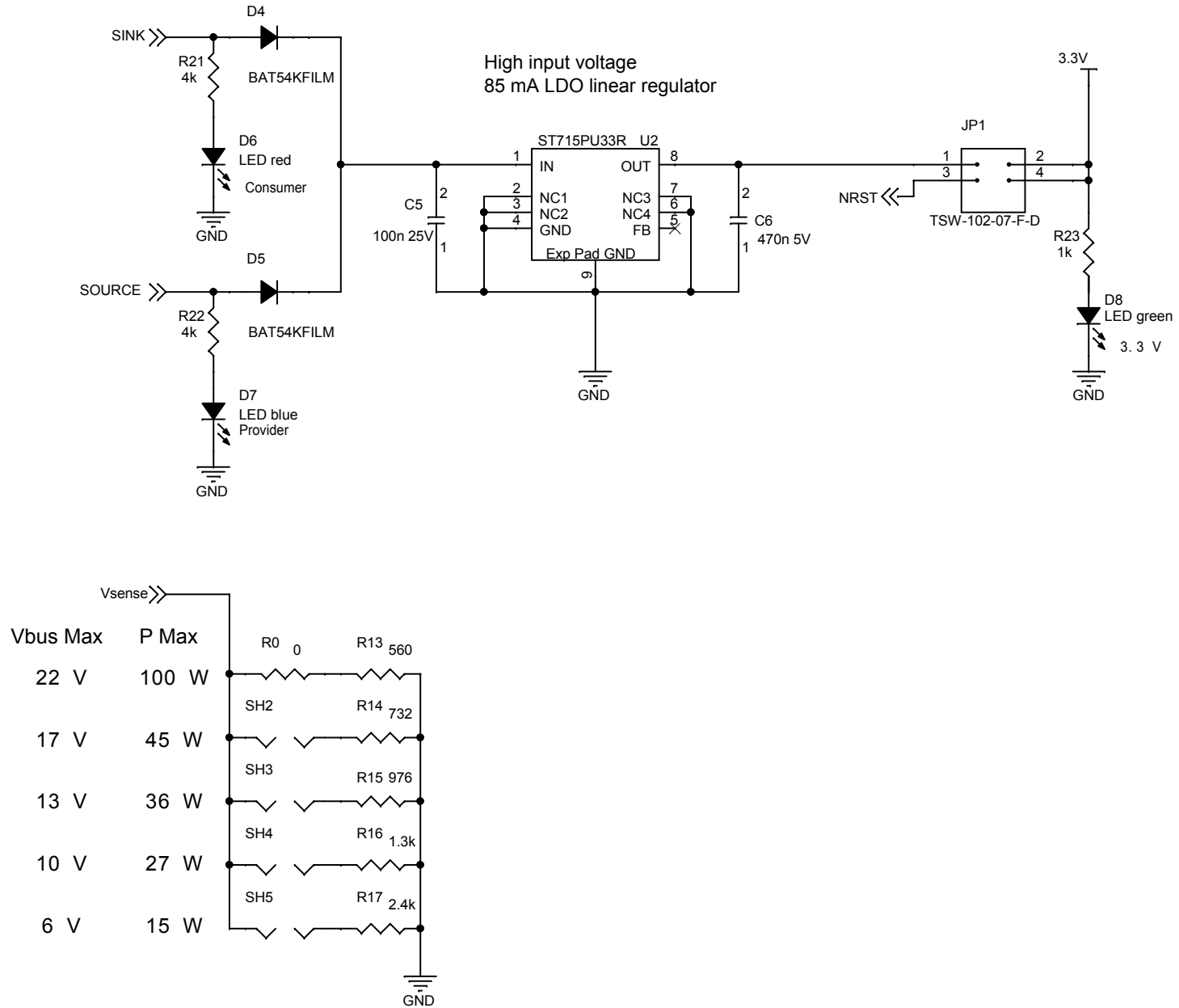
Figure 3. X-NUCLEO-DRP1M1 schematic diagram (3 of 3)
