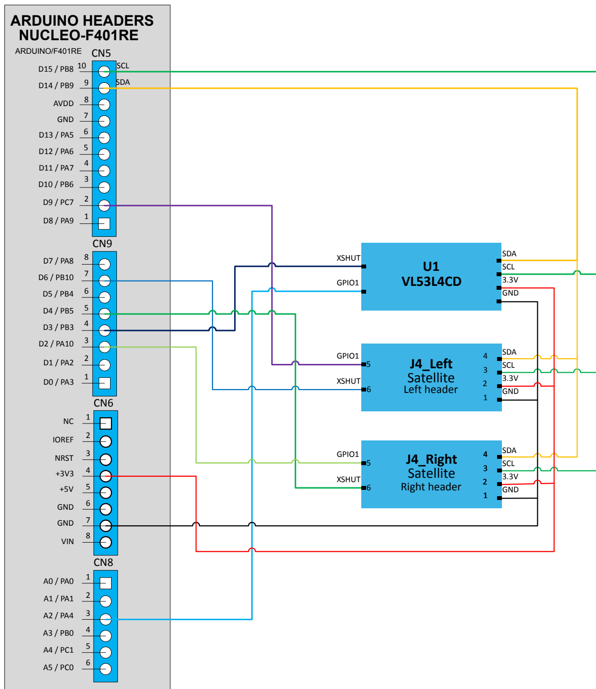
Figure 4. X-NUCLEO-53L4CD simplified schematic
