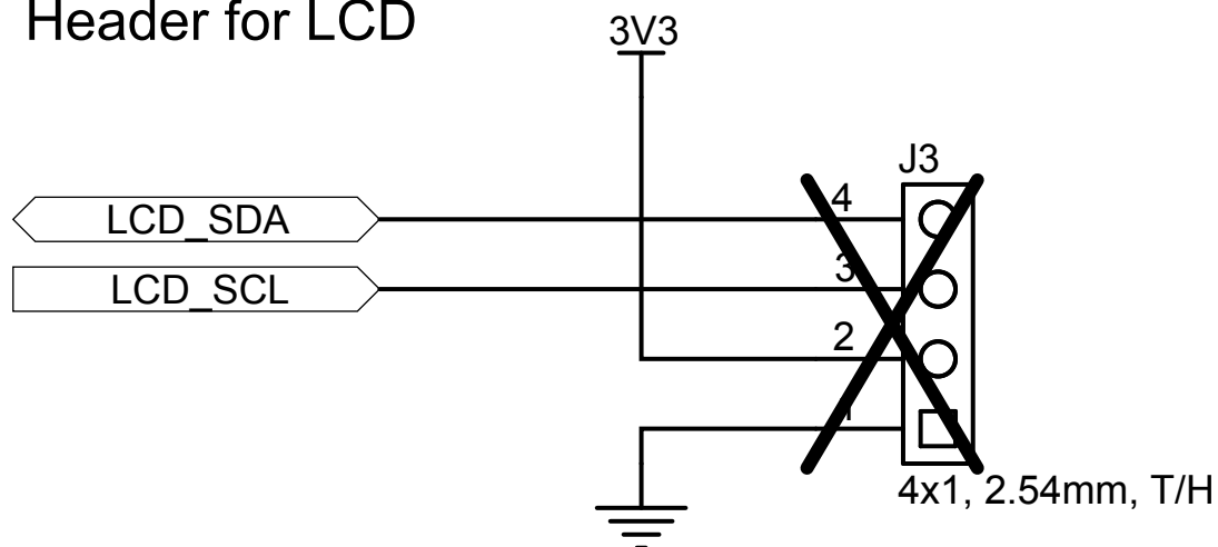
Figure 9. X-NUCLEO-53L4A1 circuit schematic (4 of 6)
