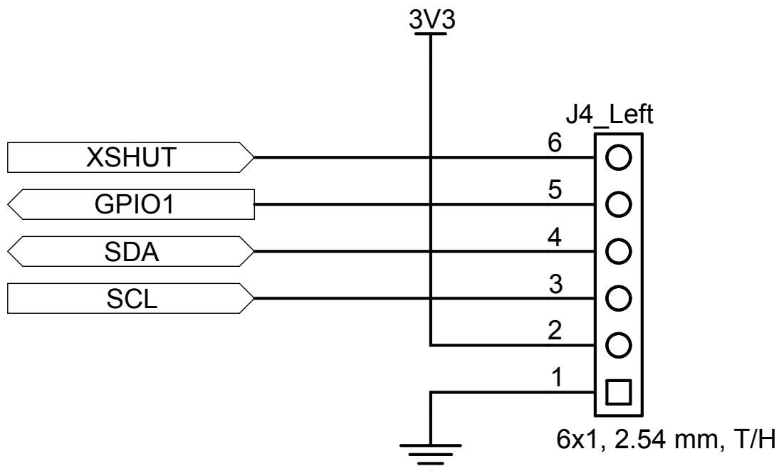
Figure 11. X-NUCLEO-53L4A1 circuit schematic (6 of 6)
