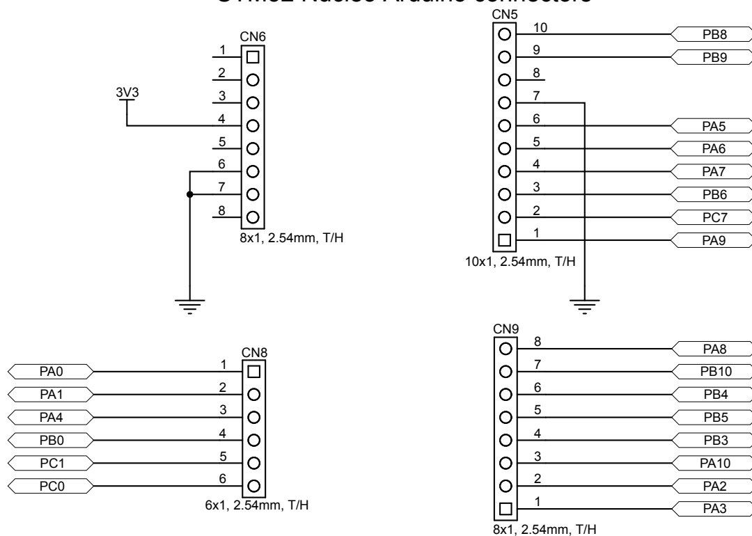
Figure 9. X-NUCLEO-53L4A1 circuit schematic (4 of 6)
