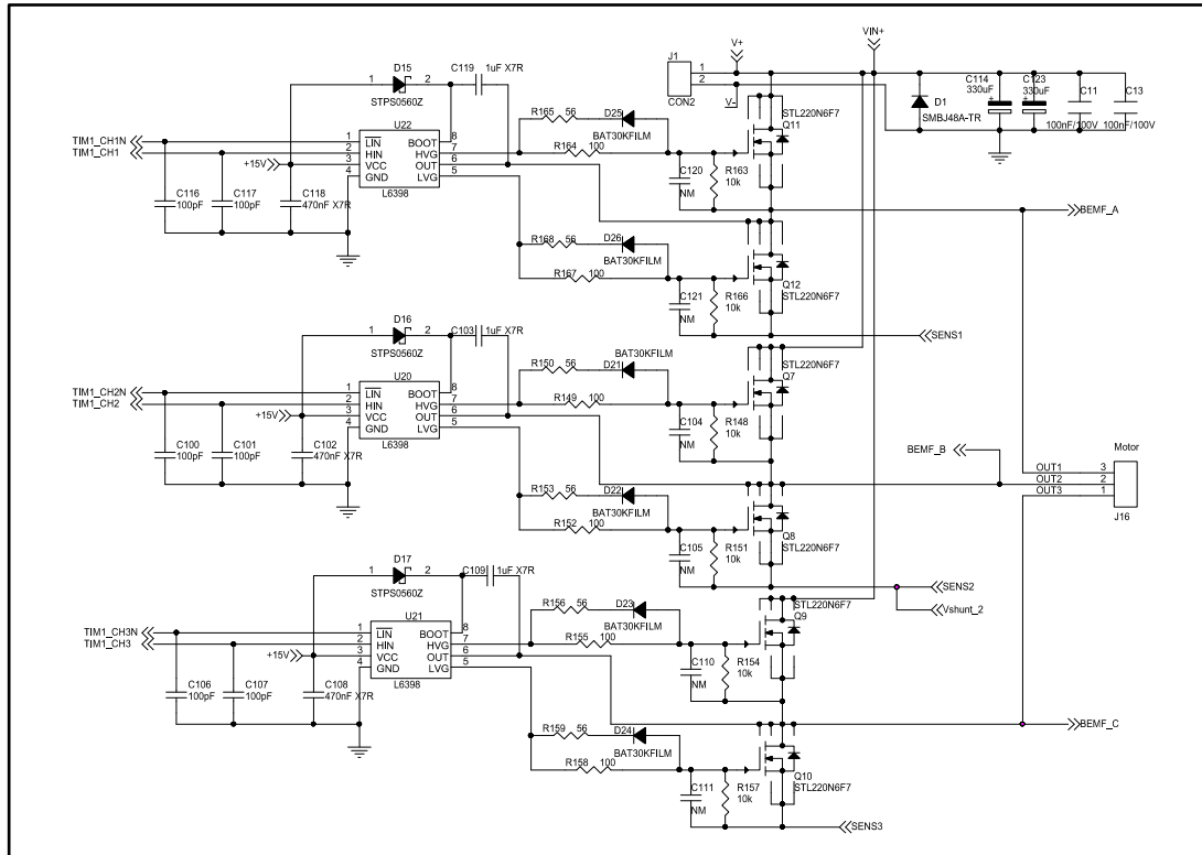
Figure 2: Schematic - Power section (2/2)
