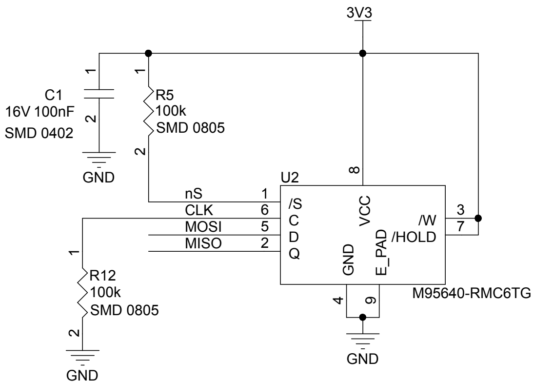
Figure 4. X-NUCLEO-IDB05A2 circuit schematic - EEPROM
