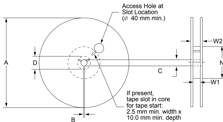
Figure 27. PowerSSO-16 reel 13"
