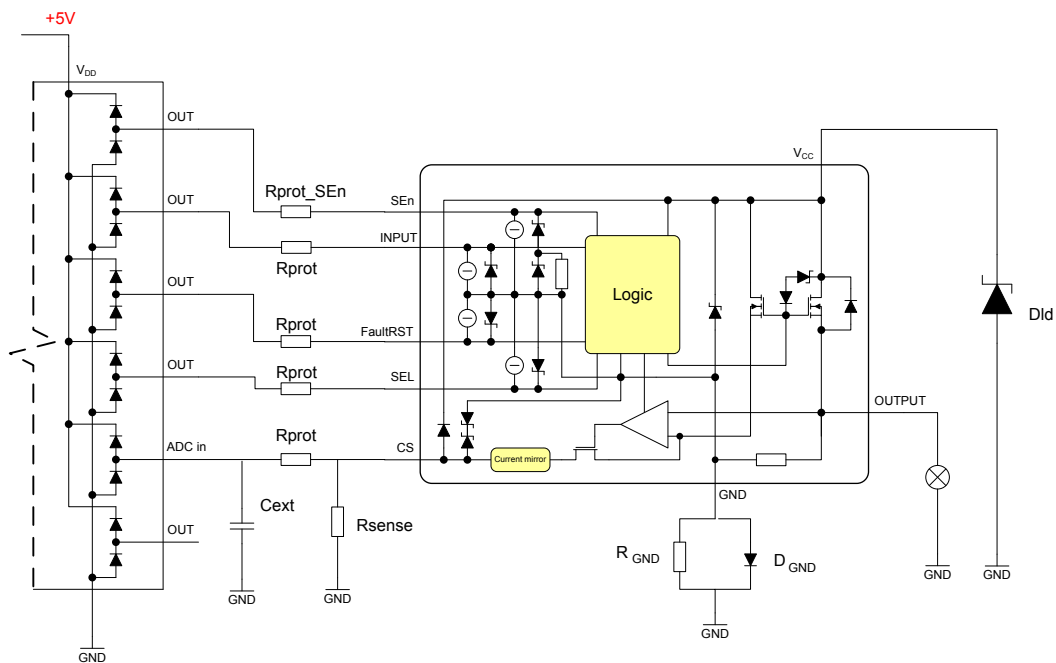
Figure 12. Application diagram
