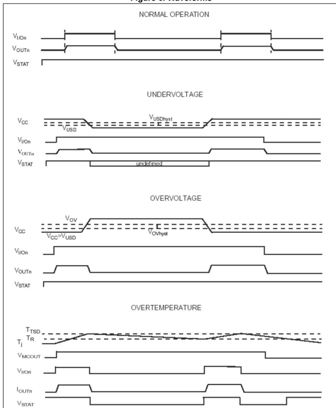
Figure 6. Waveforms
