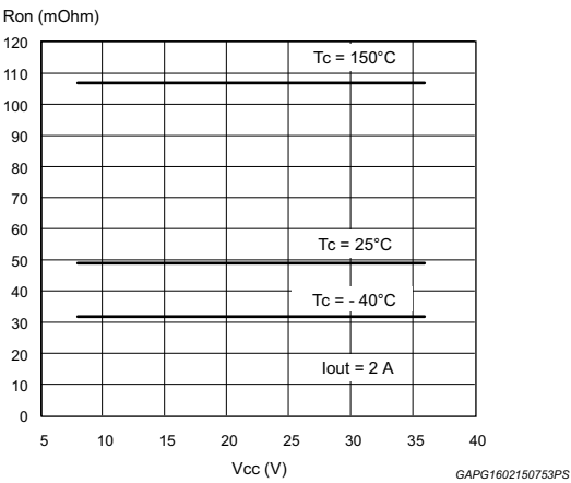
Figure 14. On-state resistance vs V_{CC}
