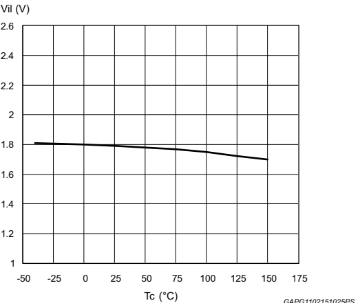
Figure 18. Input low level
