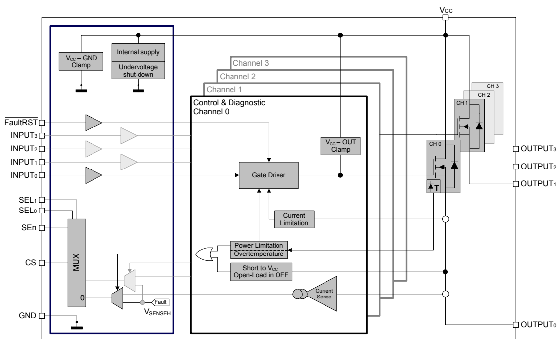
Figure 1. Block diagram
