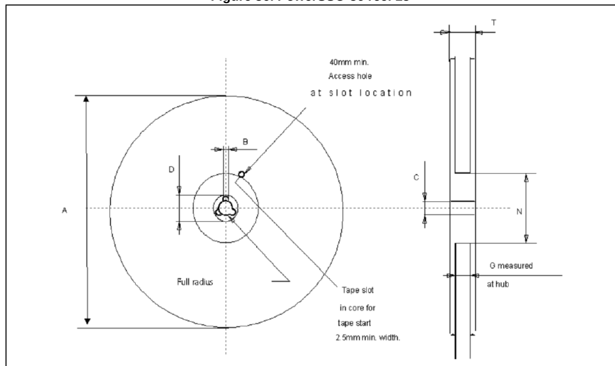
Figure 36. PowerSSO-36 reel 13"
