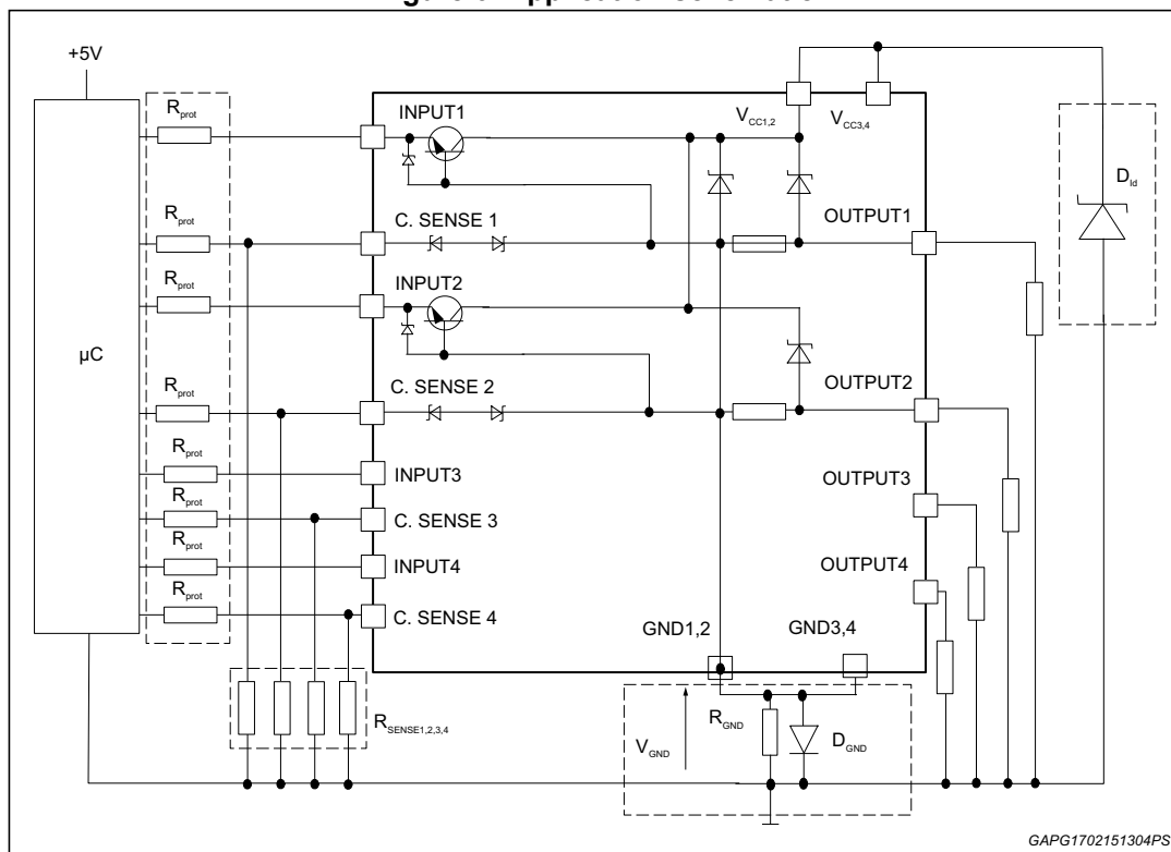
Figure 6. Application schematic
