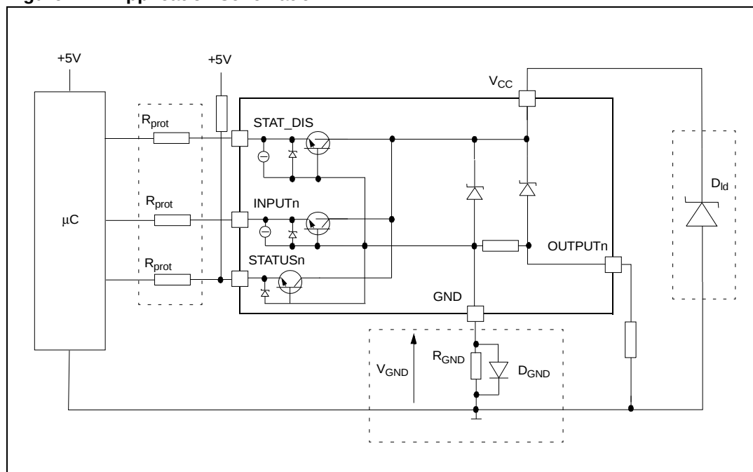
Figure 27. Application schematic
