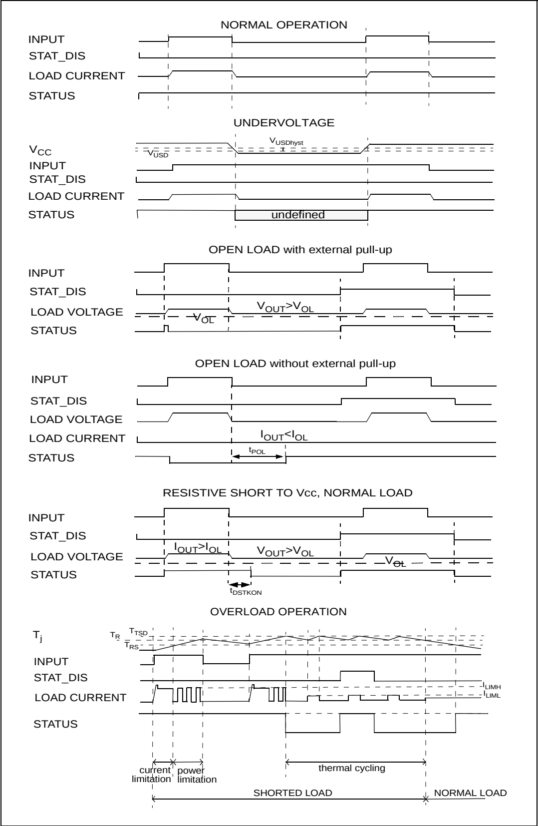
Figure 29. Waveforms
