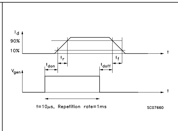
Figure 29. Waveforms
