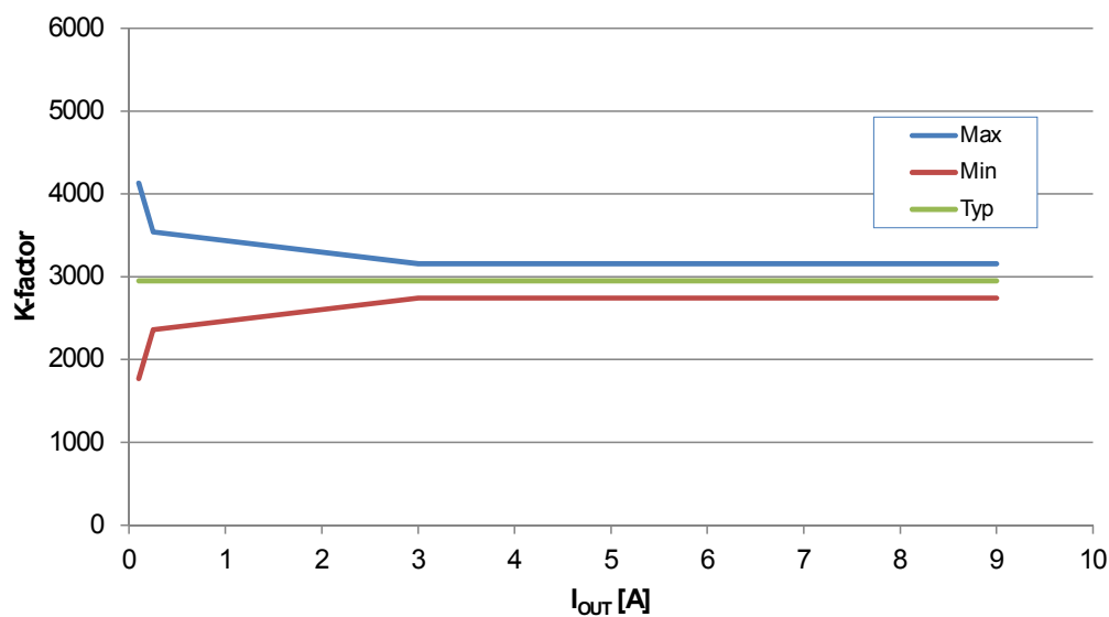
Figure 4. I_{OUT}/I_{SENSE} versus I_{OUT}
