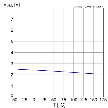
Figure 23. Undervoltage shutdown
