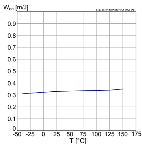
Figure 28. W_{on} vs. T_{case}
