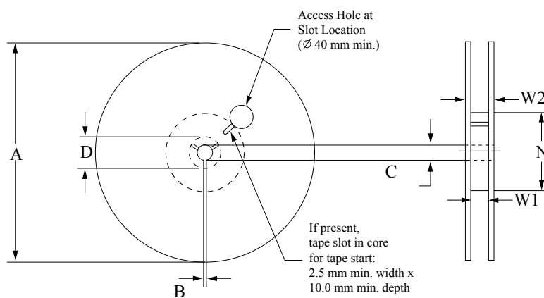
Figure 46. PowerSSO-16 reel 13"
