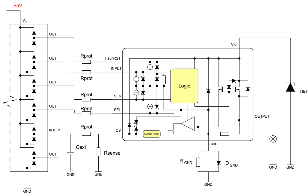
Figure 33. Application diagram
