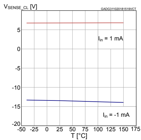
Figure 31. V_{SENSE} clamp vs. T_{case}
