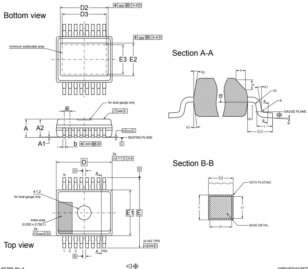
Figure 45. PowerSSO-16 package dimensions
