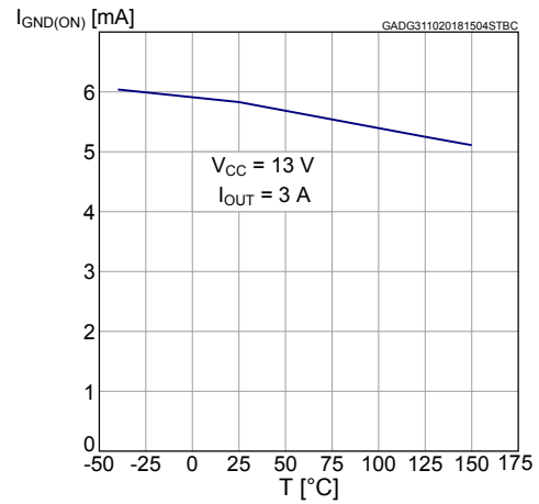
Figure 15. Standby current
