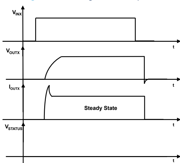
Figure 7. Switching on bulb lamp load
