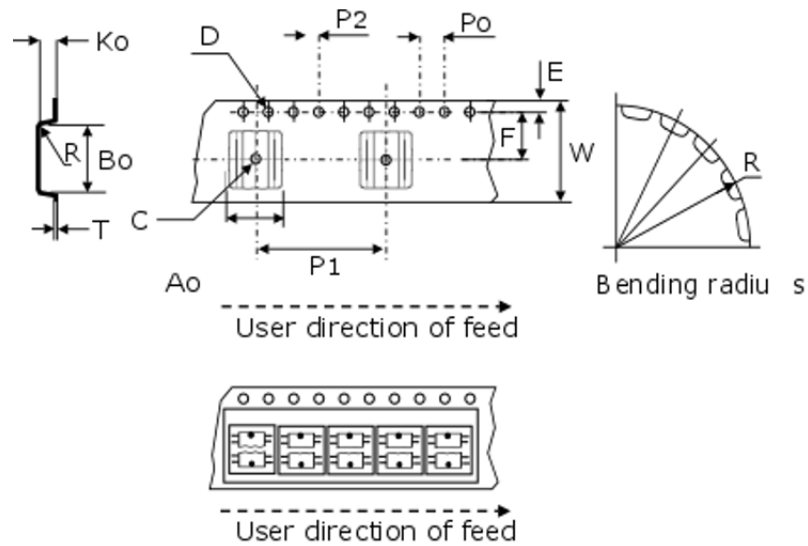
Figure 20. Tape specifications
