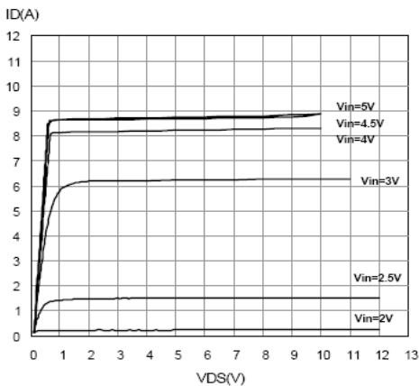
Figure 33. Output characteristics
