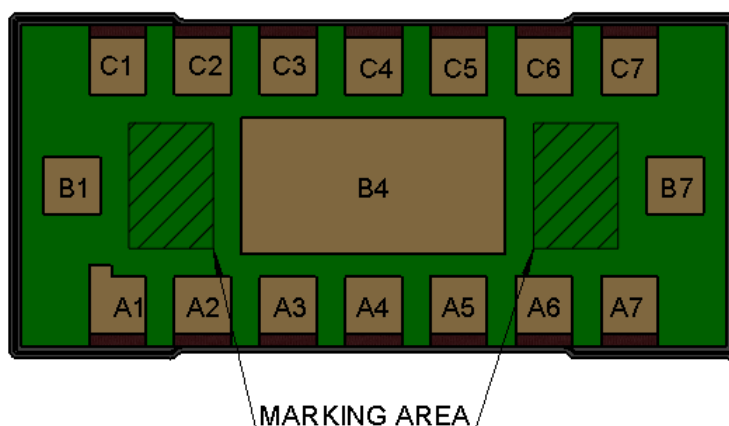
Figure 27. Product marking area
