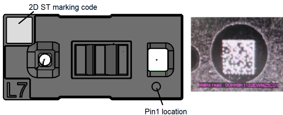
Figure 28. 2D product marking code
