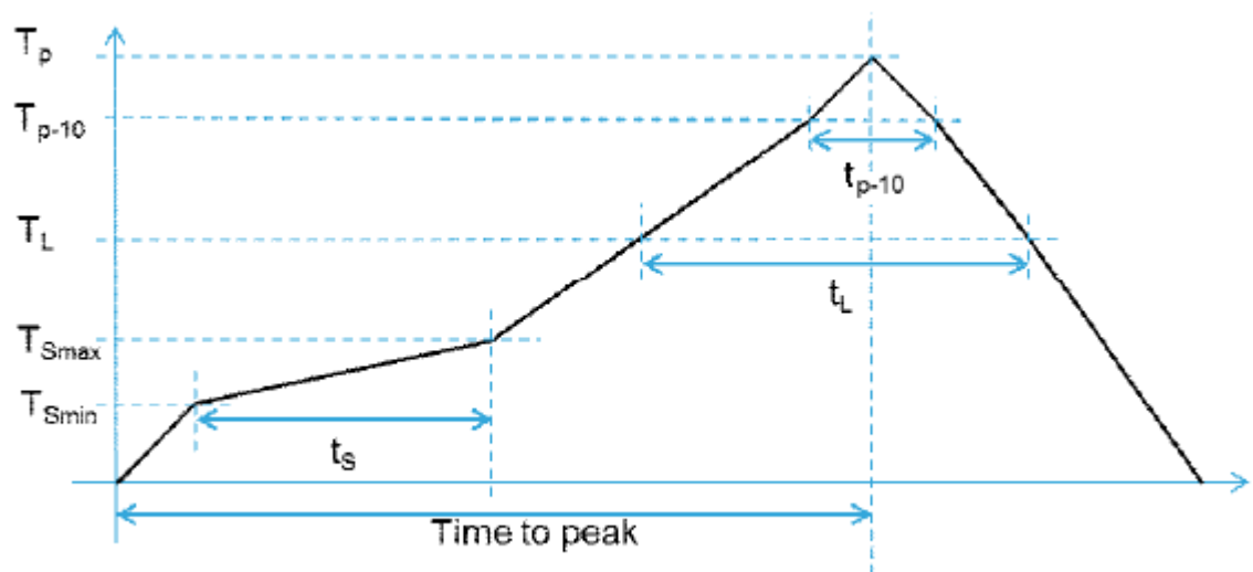
Figure 30. Solder profile
