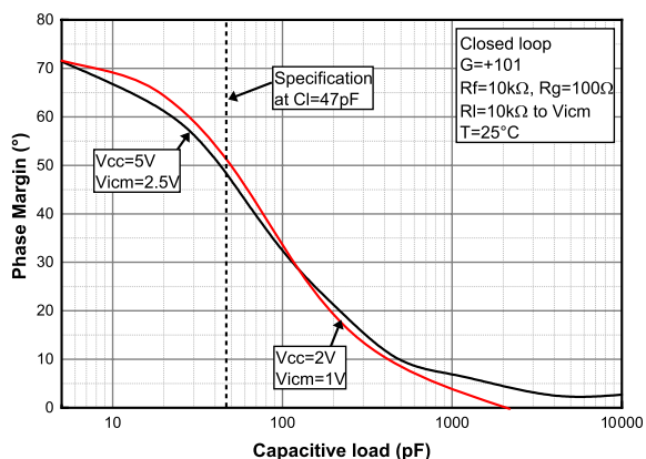
Figure 27. Phase margin vs. capacitive load
