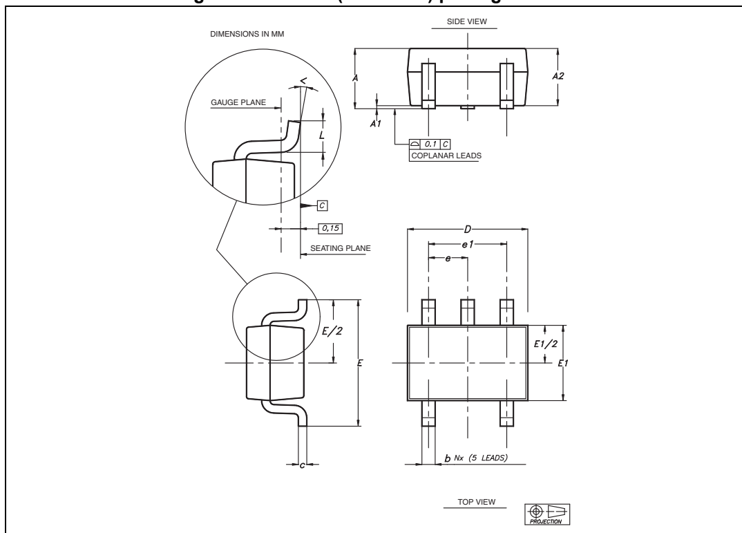
Figure 21. SC70-5 (SOT323-5) package outline
