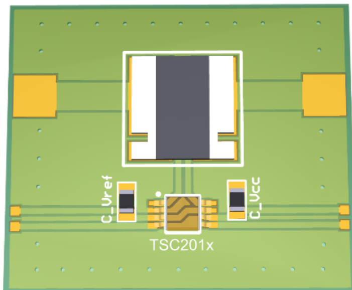
Figure 72. Recommended layout
