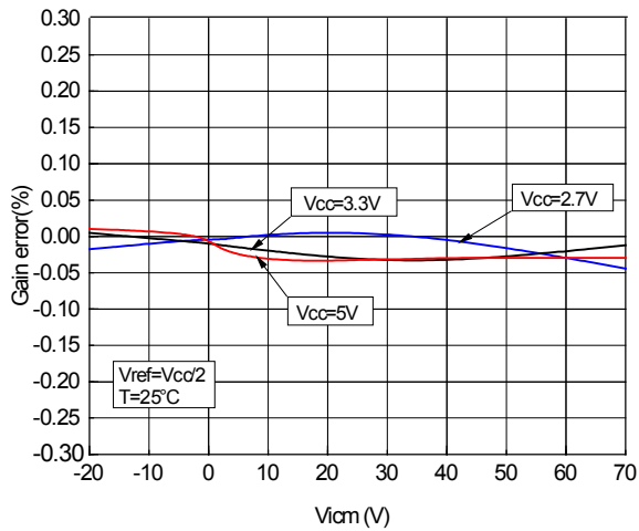
Figure 23. Gain error vs. input common mode
