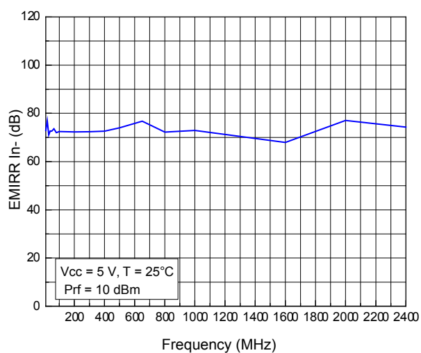
Figure 76. EMIRR on pin- (TSC2010H)
