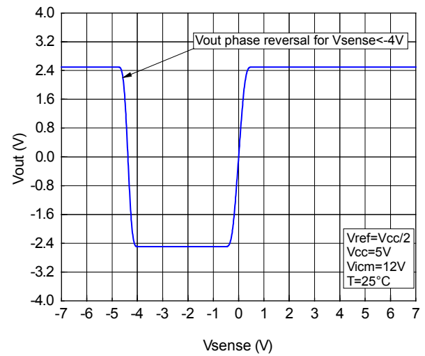
Figure 52. Output voltage vs. V_{\text{sense}} beyond the sense operating
