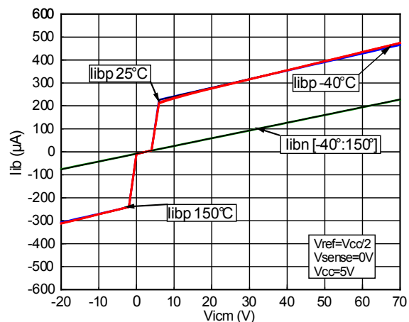
Figure 9. Input bias current vs. temperature with V_{CC} = 5\text{ V}
