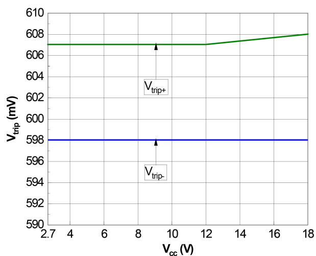
Figure 19. Comparator trip points vs. V_{\text{CC}}
