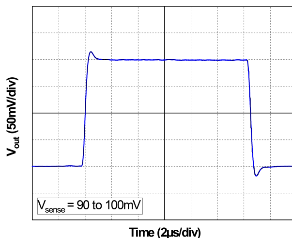
Figure 17. Step response for 90 to 100 mV V_{\text{sense}}
