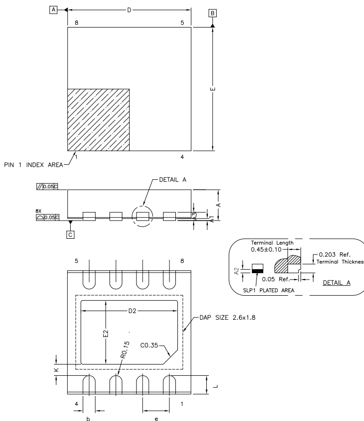
Figure 45. DFN8 3x3 package outline and mechanical data
