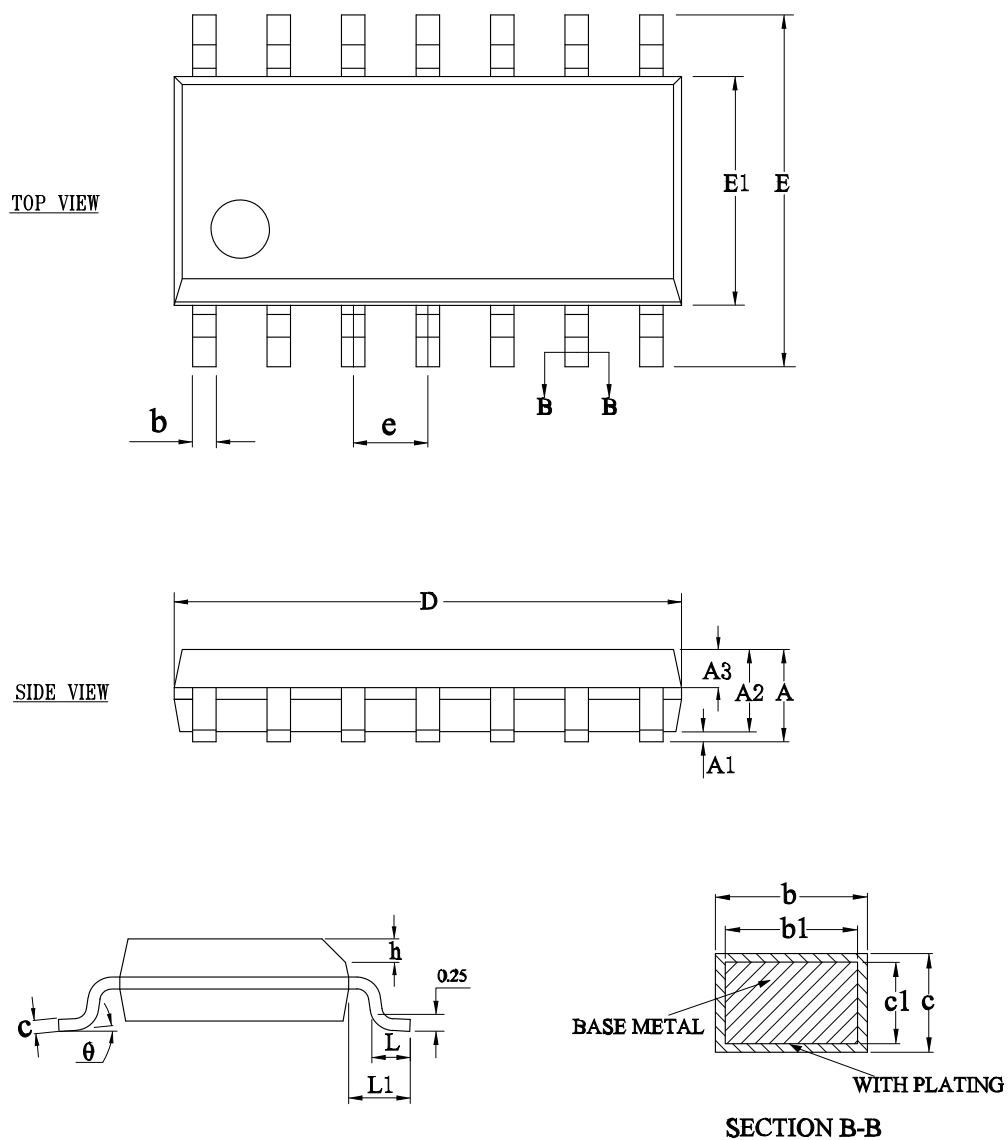
Figure 47. SO14 package outline
