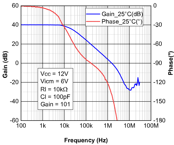
Figure 16. Bode diagram at V_{CC} = 12\text{ V}
