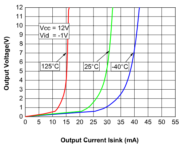
Figure 27. Output sink current vs. output voltage at V_{CC} = 12\text{ V}
