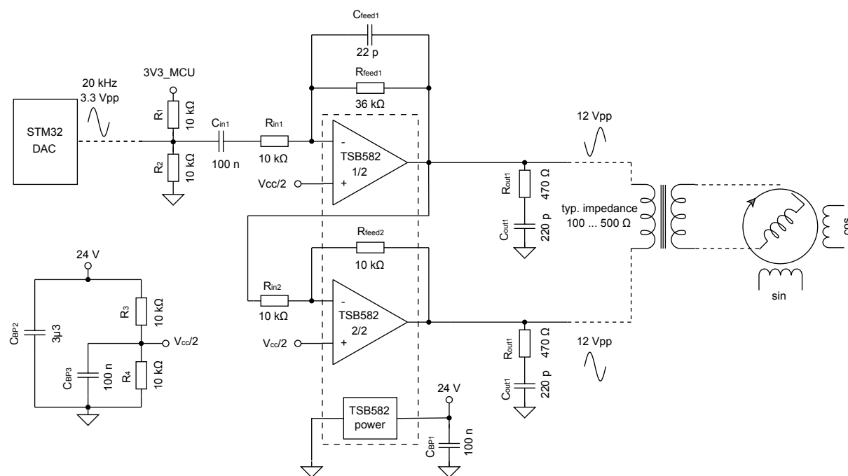
Figure 33. Rotary resolver excitation amplifier
