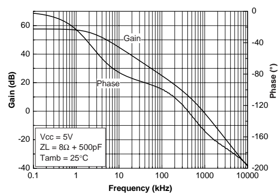
Figure 15. Open loop gain vs. frequency
