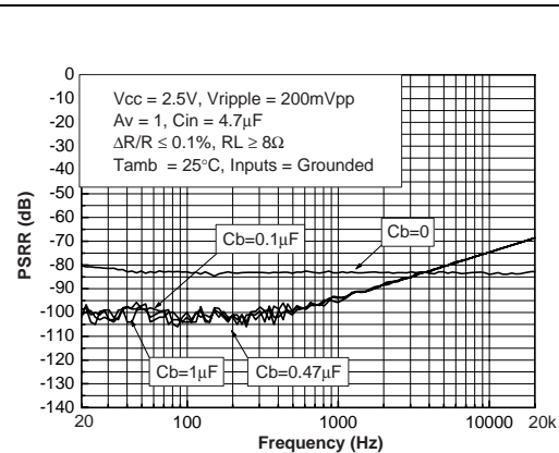
Figure 93. PSRR vs. frequency with random choice condition
