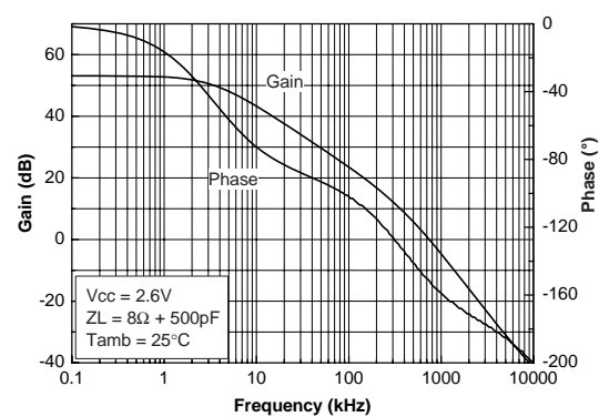
Figure 17. Open loop gain vs. frequency
