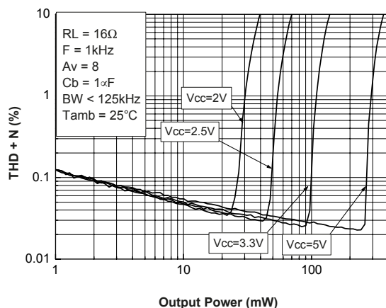
Figure 81. THD + N vs. output power R_L = 16\ \Omega , A_v = 8
