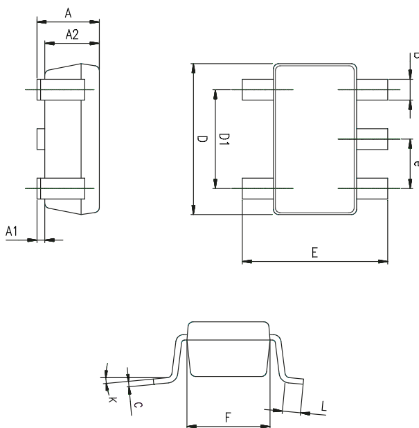
Figure 8. SOT23-5 package outline
