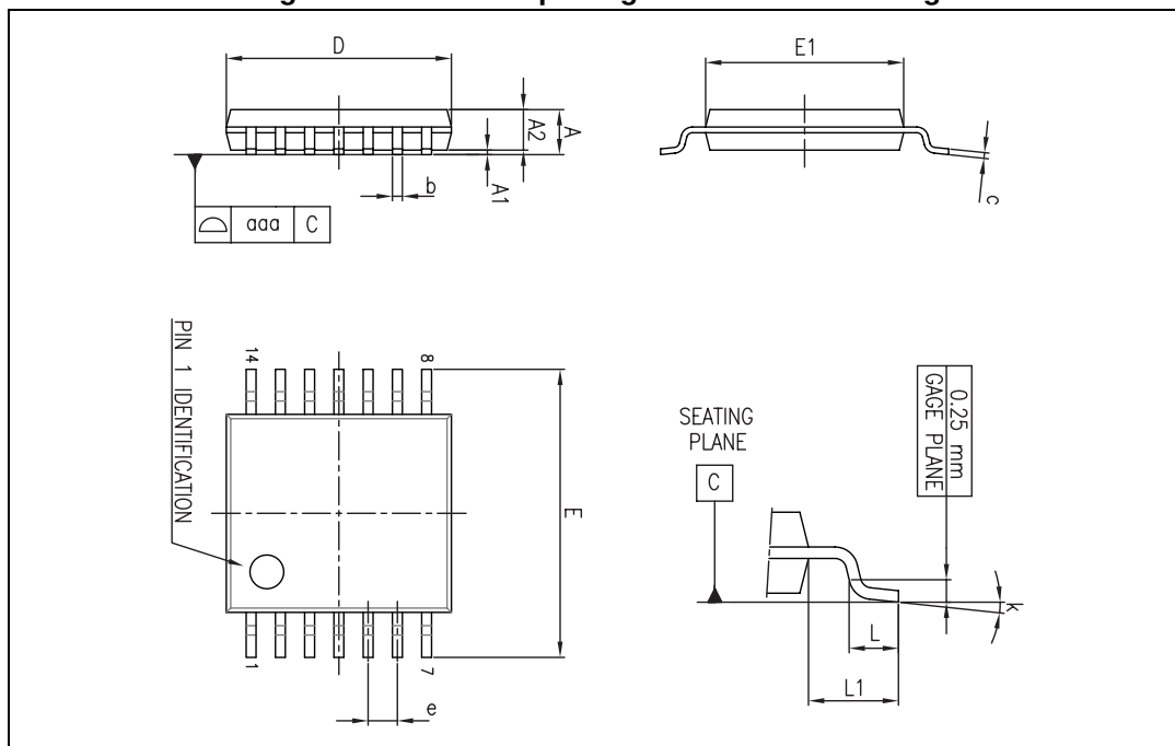
Figure 36. TSSOP14 package mechanical drawing
