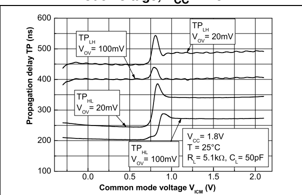
Figure 17. Propagation delay versus common mode voltage, V_{CC} = 1.8\text{ V}
