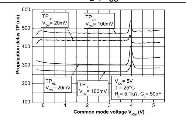
Figure 23. Propagation delay versus common mode voltage, V_{CC} = 5 V
