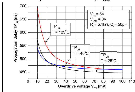
Figure 22. Propagation delay versus overdrive with positive transition, V_{CC} = 5 V
