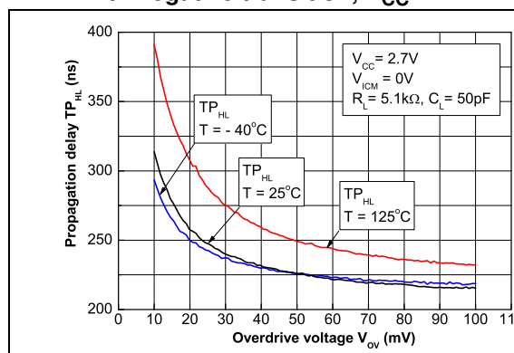
Figure 18. Propagation delay versus overdrive with negative transition, V_{CC} = 2.7\text{ V}
