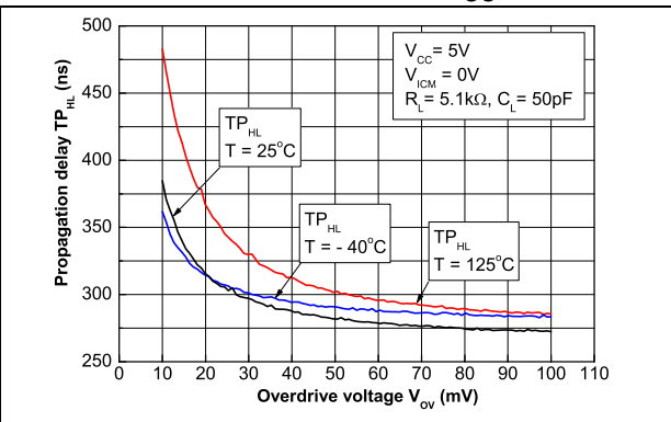
Figure 21. Propagation delay versus overdrive with negative transition, V_{CC} = 5 V
