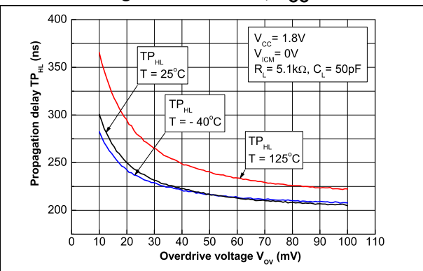
Figure 15. Propagation delay versus overdrive with negative transition, V_{CC} = 1.8\text{ V}
