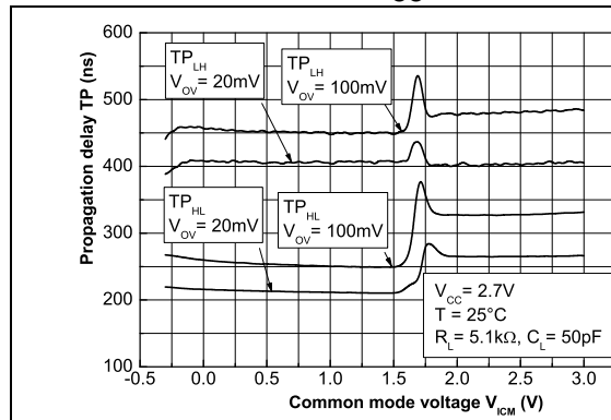
Figure 20. Propagation delay versus common mode voltage, V_{CC} = 2.7 V
