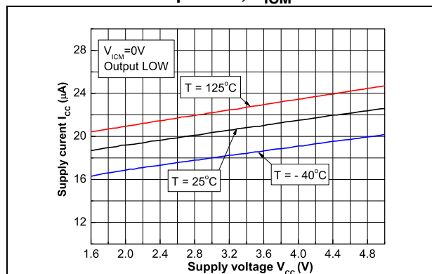
Figure 4. Supply current versus supply voltage with output low, V_{ICM} = 0 V
