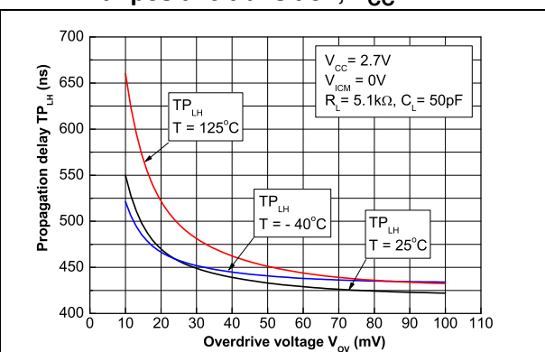
Figure 19. Propagation delay versus overdrive with positive transition, V_{CC} = 2.7\text{ V}
