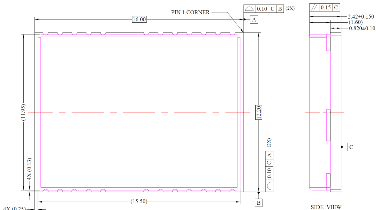
Figure 6. Mechanical specifications (Top view)
