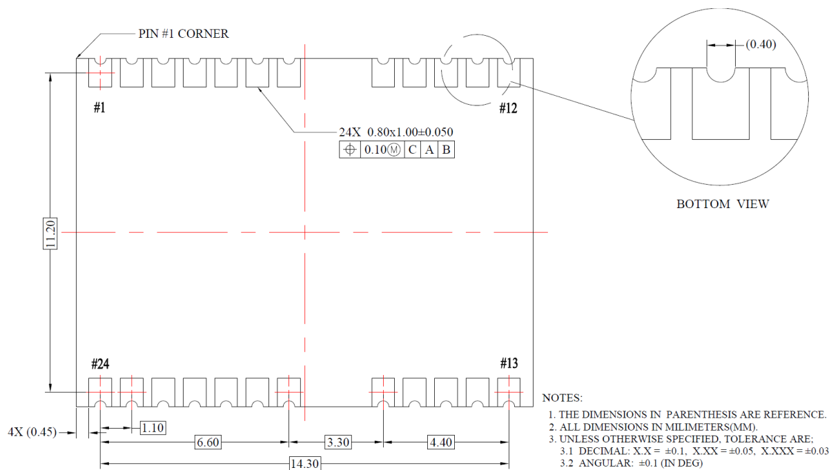
Figure 7. Mechanical specifications (bottom view)
