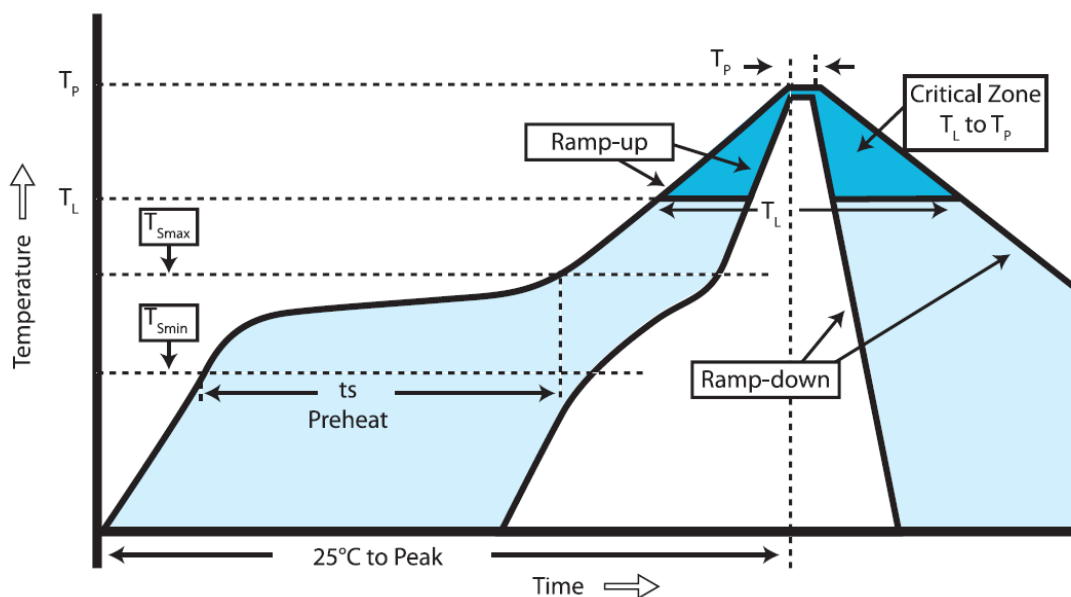
Figure 10. Soldering profile
