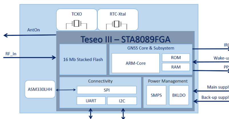
Figure 1. Block schematic
