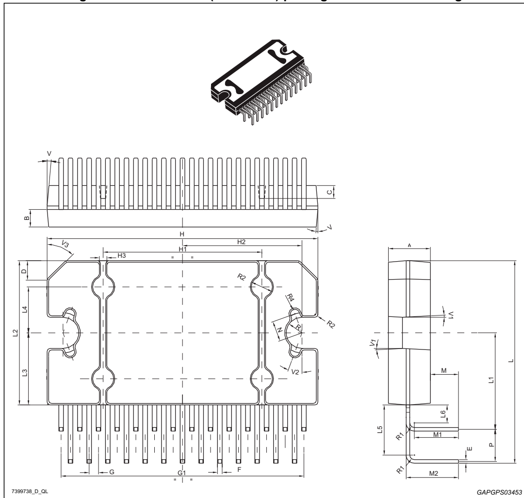
Figure 42. Flexiwatt 27 (horizontal) package mechanical drawing
