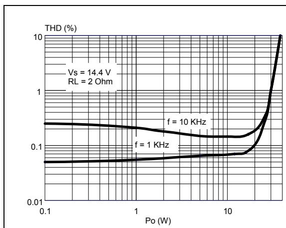
Figure 8. Distortion vs. output power (2 \Omega )
