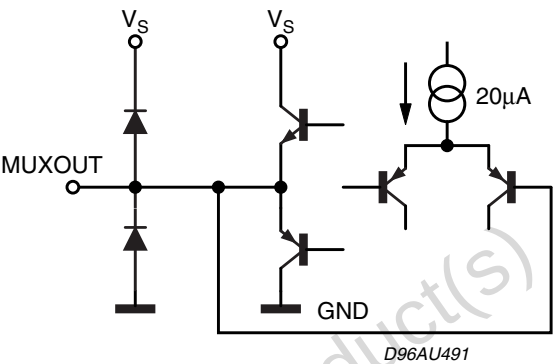
Figure 19. Pins 12, 15
