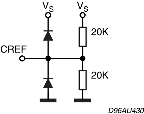
Figure 18. Pins 4, 5
