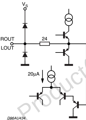
Figure 20. Pins 6, 7, 8, 9
