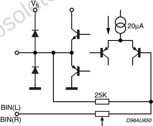
Figure 21. Pins 13, 14
