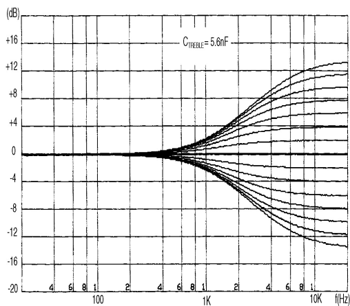
Figure 10. Treble response
