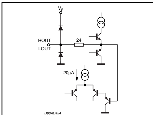
Figure 21. Pins 8, 9
