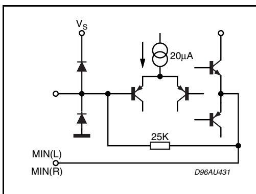
Figure 23. Pins 10, 17
