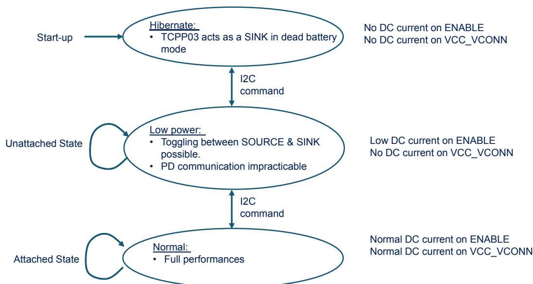
Figure 8. Power modes process
