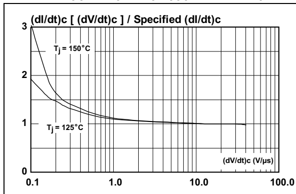
Figure 11. Relative variation of critical rate of decrease of main current (di/dt)_c versus reappplied (dV/dt)_c (typical values)
