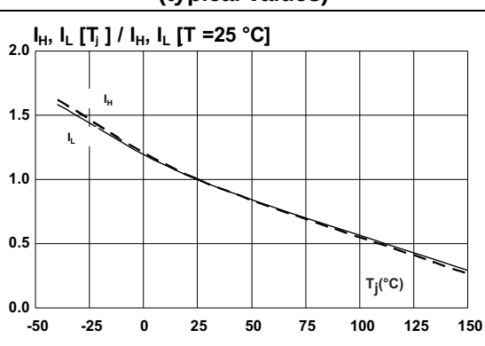
Figure 10. Relative variation of holding and latching current versus junction temperature (typical values)
