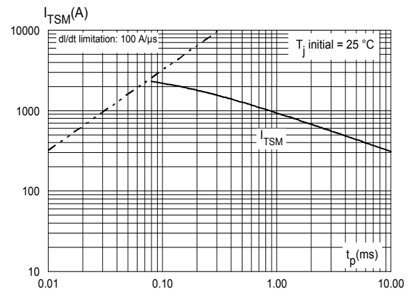
Figure 10. Non repetitive surge peak on-state current for a sinusoidal pulse with width t_p < 10 ms
