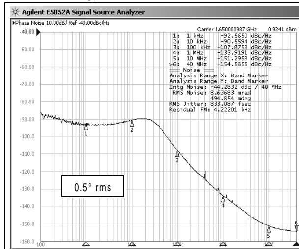
Figure 7. VCO A (div. by 2 output) closed loop phase noise at 1.65GHz (F_{STEP}=200\text{kHz}; F_{PFD}=400\text{kHz}; I_{CP}=2\text{mA})
