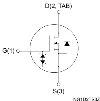
TO-247
