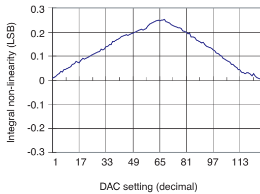
Figure 17. Integral non-linearity vs. DAC setting
