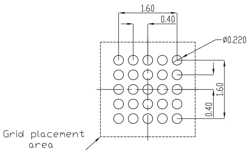
Figure 13. WLCSP (2.6x2.6x0.5) recommended footprint
