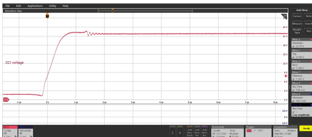
Figure 4. Short-to- V_{BUS}
