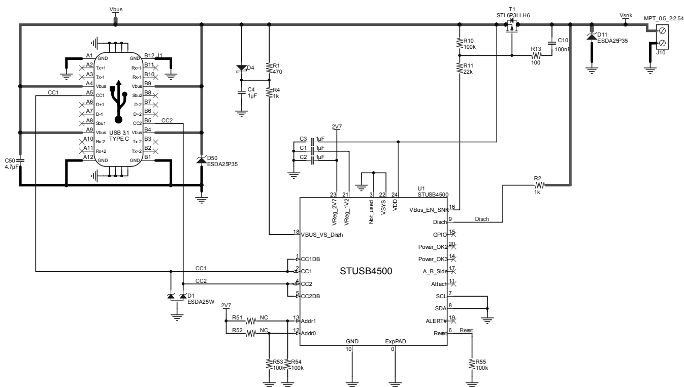
Figure 9. STUSB4500 schematic
