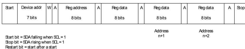
Figure 6. Write operation
