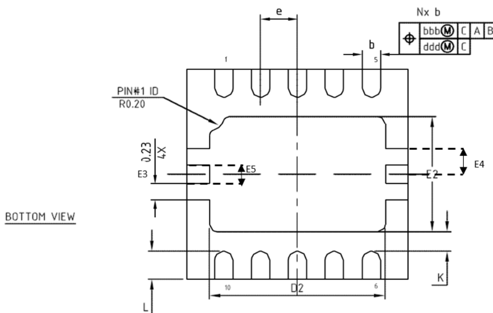
Figure 26. DFN10 package outline (bottom view)
