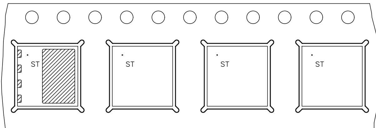
Figure 12. PowerFLAT™ 8x8 HV package orientation in carrier tape
