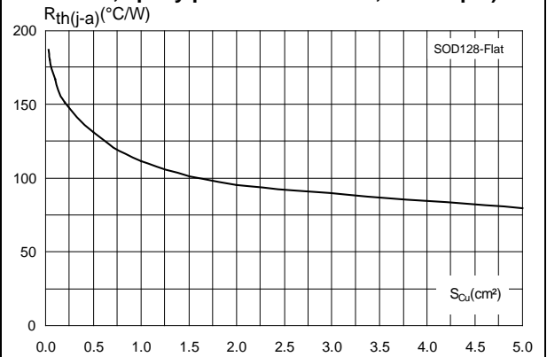
Figure 8: Thermal resistance junction to ambient versus copper surface under each lead (typical values, epoxy printed board FR4, e_{Cu}=35 \mu m )
