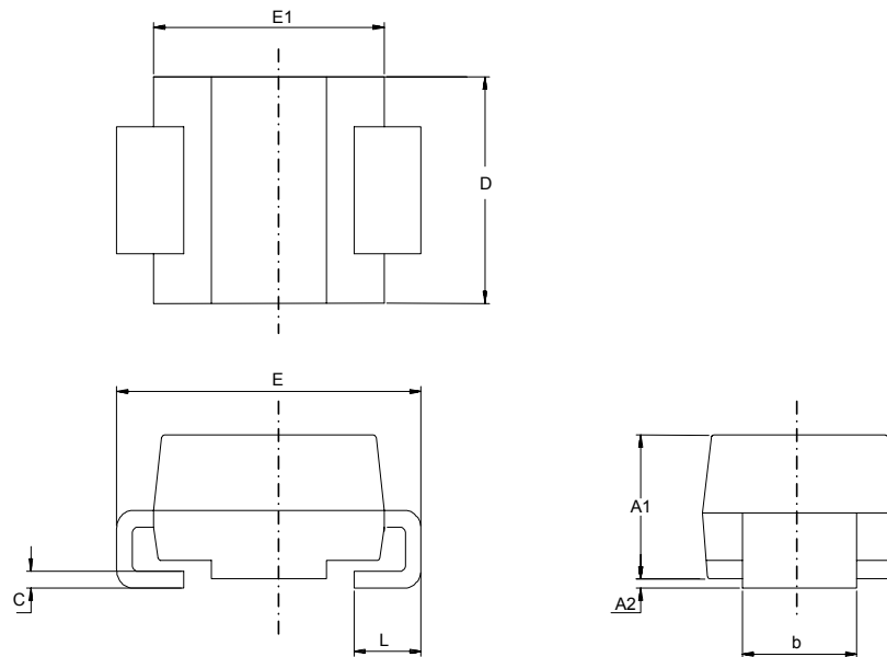
Figure 12. SMA package outline
