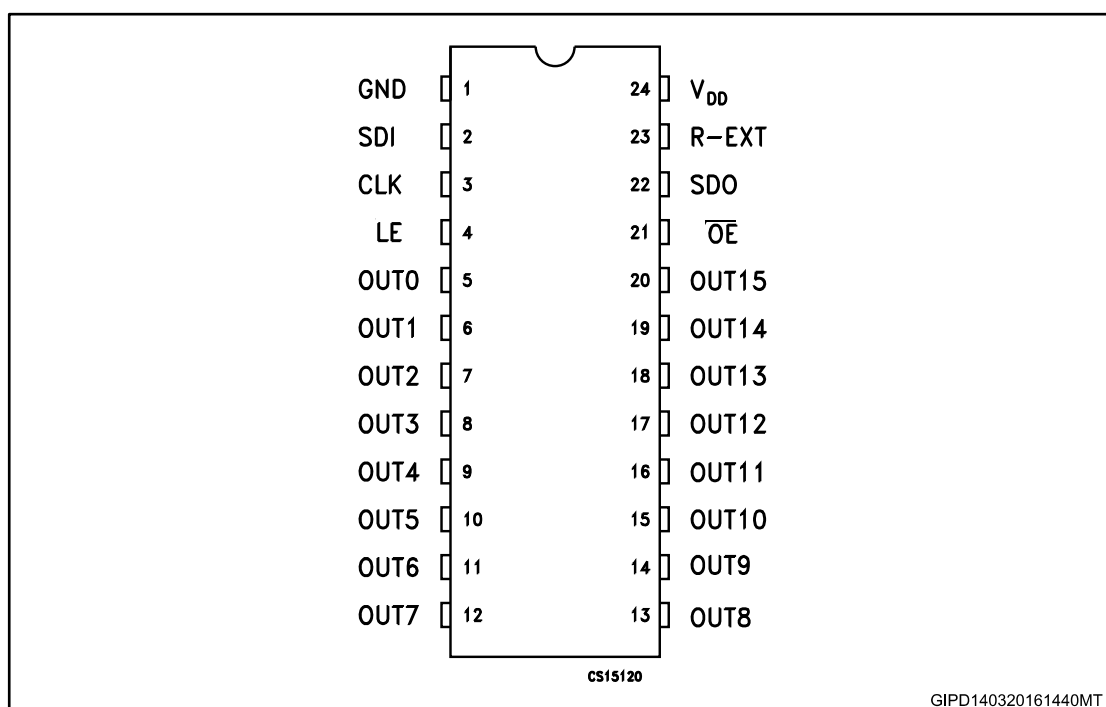
Figure 1: Pin connection
