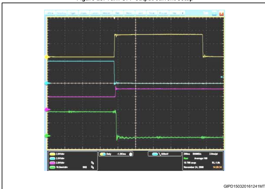
Figure 18: Turn OFF output current setup
