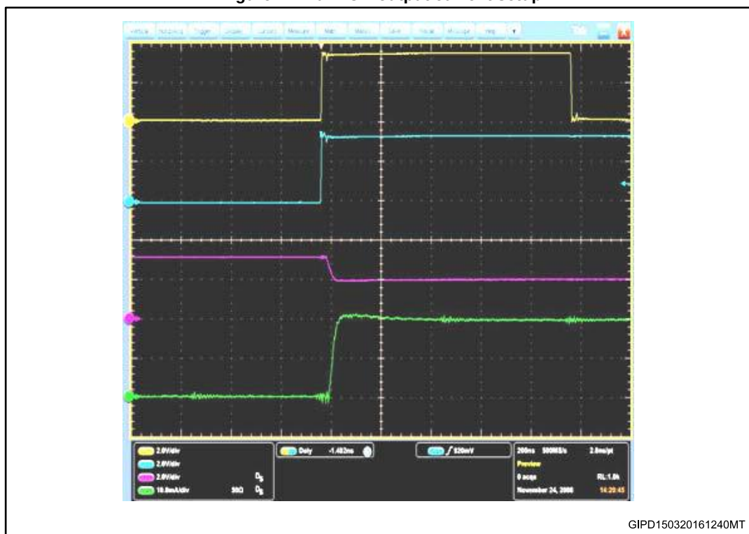
Figure 17: Turn ON output current setup
