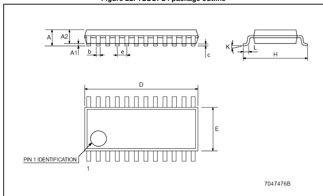
Figure 21: TSSOP24 package outline
