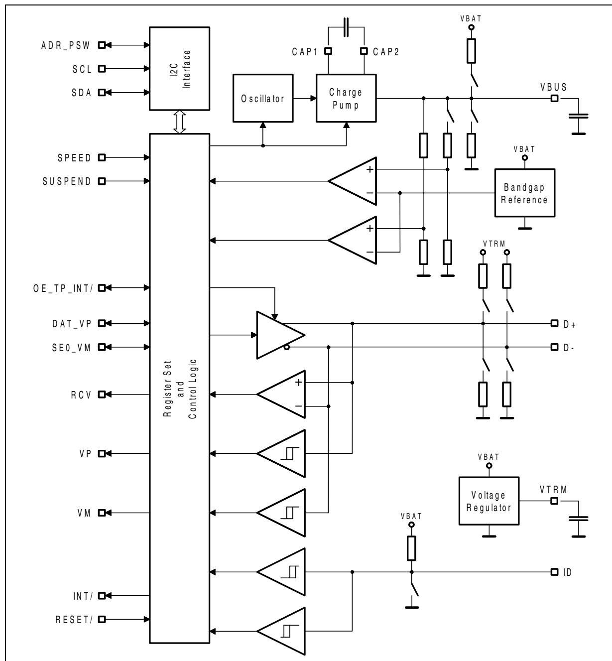
Figure 11. Block diagram
