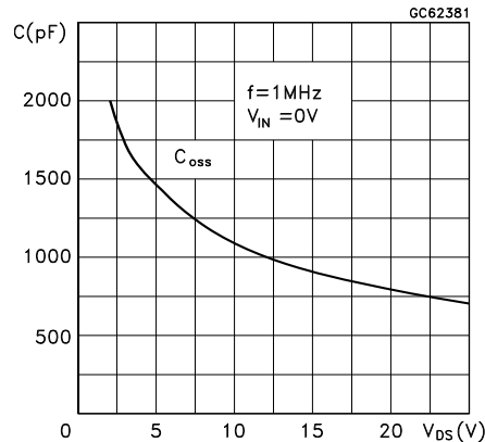
Figure 19. Capacitance variations
